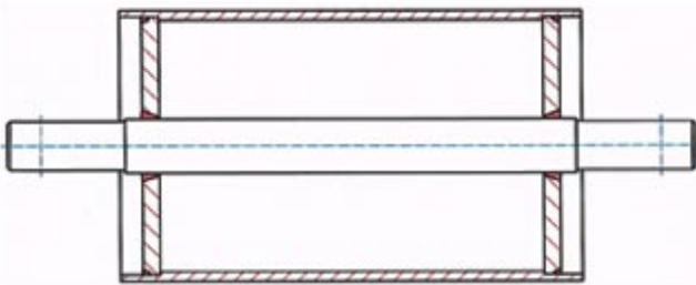
Idler pulley - welded design (UTS)
